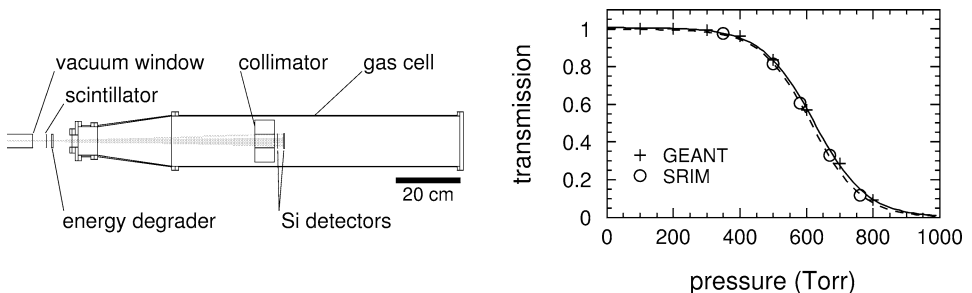
Fig. 1. Basic layout of the experimental setup (left panel). The right panel shows a comparison of transmission curves calculated by SRIM and GEANT for 100 MeV/u ^{36}\text{Ar} in 50 cm He gas. A 4.135 mm Al energy degrader was used for the simulations. The width parameter of a Woods-Saxon fit to the SRIM distribution (dashed line) is 76 Torr, while GEANT (solid line) yields 78 Torr, which is a good agreement.
