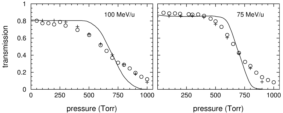
Fig. 2. Transmission curves obtained with beams of ^{36}\text{Ar} at 100 MeV/nucleon (left panel) and 75 MeV/nucleon (right panel). The experimental data (circles) are shown together with the results of the GEANT calculation (cross-hairs). The solid curves correspond to calculations with no energy spread in the primary beam.
