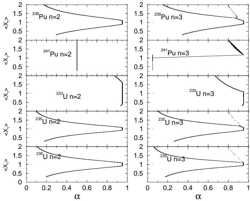
Figure 2.6: The values of \alpha that minimized \delta(\alpha_{min}, \overline{\Gamma}_1^0) for a given \overline{\Gamma}_1^0 vs. the corresponding \overline{\Gamma}_1^0 (labelled as \langle X_1 \rangle on the y-axis). The values of \overline{\Gamma}_1^0 taken from Fig. (2.5) were used here to get the values of \alpha that best fit the data.
