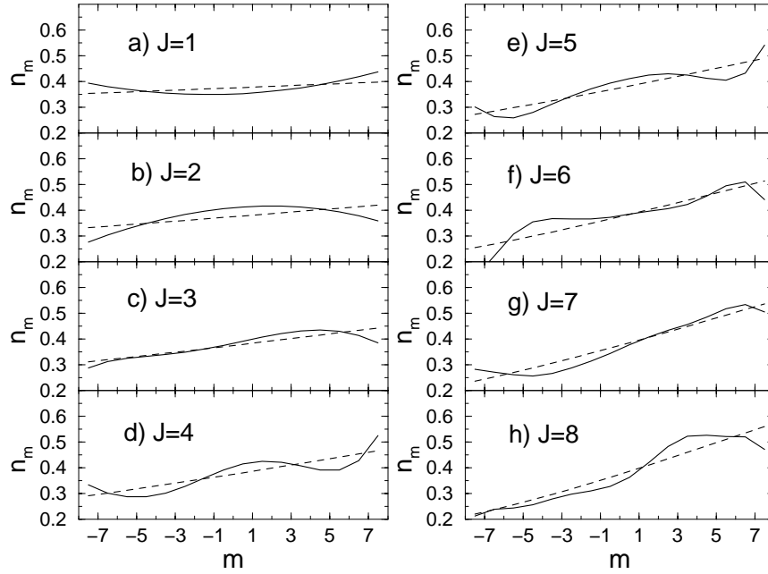
Figure 4.7: The single-particle occupation numbers n_m averaged over the lowest energy spin J wave functions of the 1417 out of 2000 (70%) spectra with J_0 = 0 (solid line), compared to the simplest theoretical expression (4.10) (dashed line)
