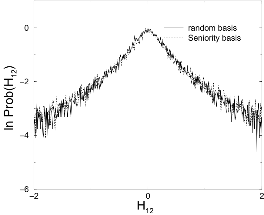
Figure 3.18: The probability distribution P(H_{ij}) of the off-diagonal matrix elements of the 2 \times 2 J = 0 block of the N = 4 , j = 11/2 Hamiltonian in the |JM\rangle basis but this time rescaled with an alternative prescription to that of Fig. 3.17.
