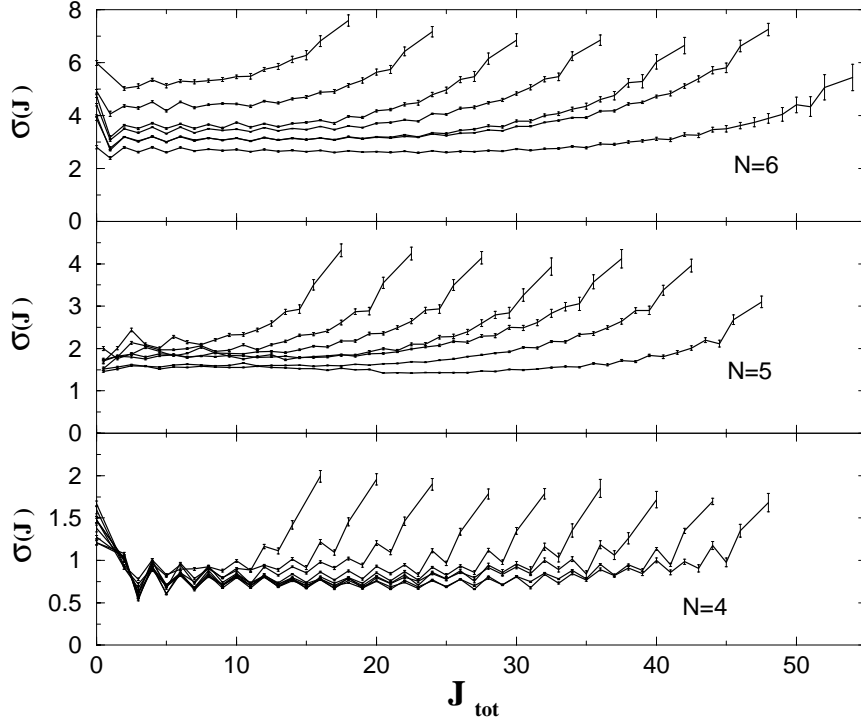
Figure 3.13: The standard deviation of the level density \rho_J(E) of states with total angular momentum J_{Total} for all the systems. The values of j start at 11/2 and increase by one as the lines get progressively longer.
