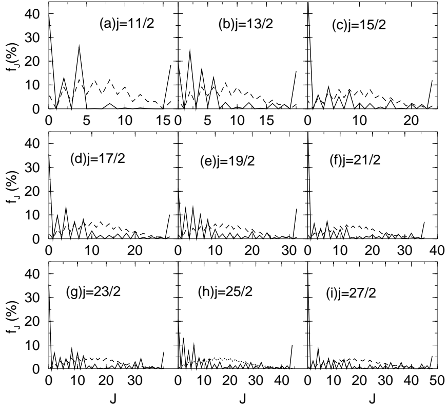
Figure 3.3: The distribution f_J of ground state spins J_0 for various systems of N = 4 particles.
