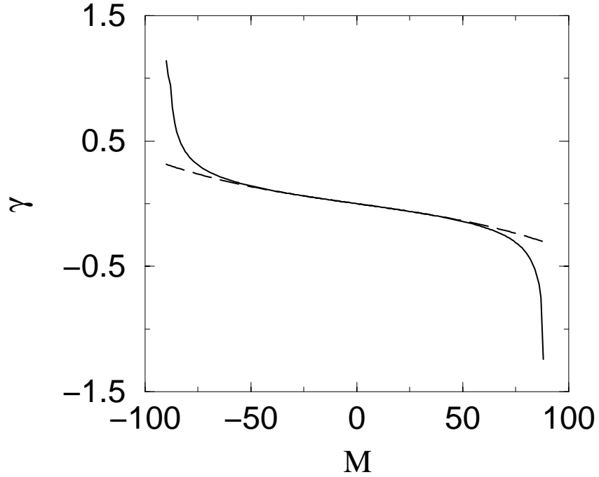
Figure 4.2: The cranking frequency \gamma vs. M for N=10 and j=27/2 . Solid and dotted lines correspond to exact and approximate values, respectively. This gives an indication of the range of validity of the expansion that gives eq. (4.14).
