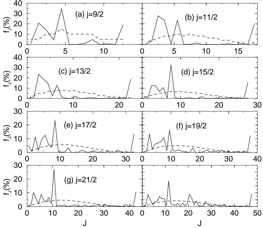
Figure 3.4: The distribution f_J of ground state spins J_0 for various systems of N = 5 particles.
