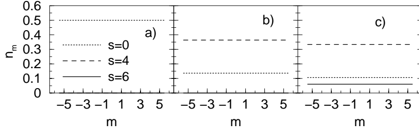
Figure 3.20: The contribution to n_m for the states S = 0 , N = 6 (a), S = 4 , N = 6 (b) and S = 6 , N = 6 (c) from Slater determinants of various seniority; here j = 11/2 . Note that for J = 0 , n_m is independent of m .
