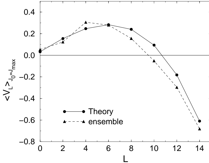
Figure 4.4: The mean values of V_L for the subsets of V_L that result in J_0 = J_{max} ground states. The theory, solid line, agrees with the ensemble average values, dashed line. Here N = 4 and j = \frac{15}{2} .
