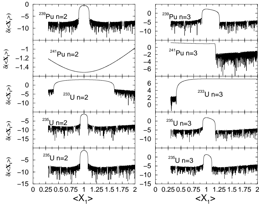
Figure 2.5: The minimum \ln \delta(\langle X_1 \rangle) vs. \langle X_1 \rangle , (here \Gamma_1^0 is written as \langle X_1 \rangle ). The left hand panels correspond to the second ( n = 2 ) moment of the data, and the right hand panels correspond to the third ( n = 3 ) moment of the data.
