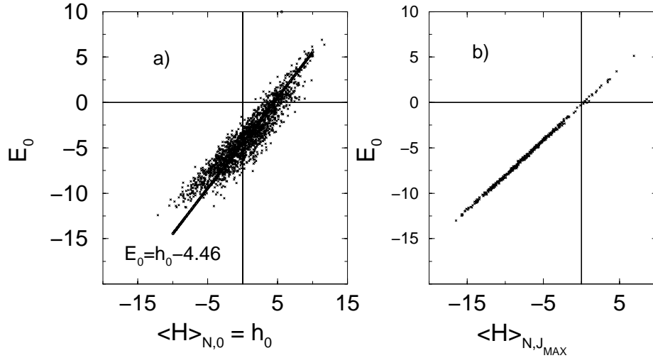
Figure 4.5: Ground state energies E_0 for J_0 = 0 ,(a), and J_0 = J_{max} ,(b), vs. predictions of the statistical model, eq. (4.16). Here N = 6 and j = 17/2 . The theoretical energies are fit to a straight line, included in (a).
