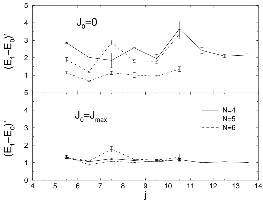
Figure 3.10: The ensemble average ground state energy gaps for all values of N and j .
