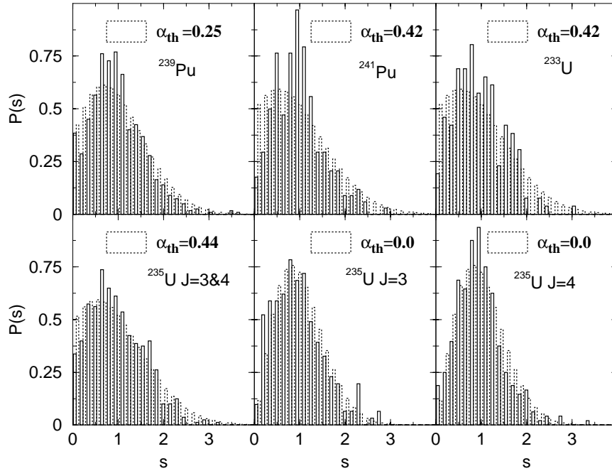
Figure 2.1: The level spacing distribution for each data set. For the ^{235}\text{U} data only the first 544 levels were included and an analysis was performed for the J = 3 and 4 resonances taken together and separately.
