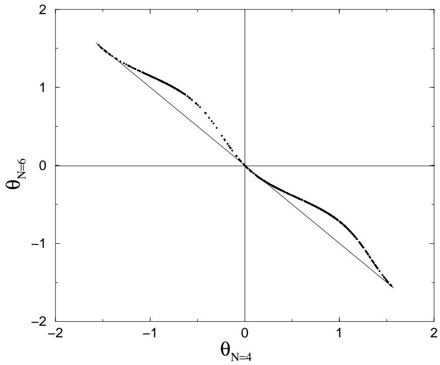
Figure 3.24: The strong correlation between the angle the spin-0 ground states make in the two-dimensional N = 4, J = 0 subspace, \theta_{N=4} and N = 6, J = 0 subspace, \theta_{N=6} . The states are eigenstates of Hamiltonians with the same interaction parameters.
