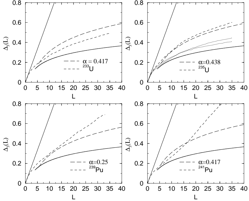
Figure 2.3: The \Delta_3(L) statistic for the data sets. The solid lines in each plot are the RMT results for spectra with the Poissonian level spacing distribution, \Delta_3(L) = L/15 , and for the GOE (lower logarithmic curve Eq. (2.4)). The long-dashed line in each plot corresponds to the RMT prediction for a superposition of two sequences in the proportions \frac{2J_1+1}{(2J_1+1)+(2J_2+1)} .
