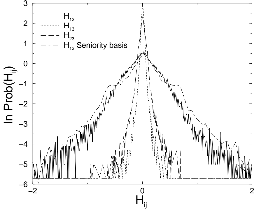
Figure 3.16: The probability distribution P(H_{ij}) of the off-diagonal matrix elements of the 3 \times 3 J = 0 block of the N = 6 , j = 11/2 Hamiltonian in the |JM\rangle basis. Except where the seniority basis is specified the basis has been randomly chosen. Note the shoulders on P(H_{ij}) in the seniority basis.
