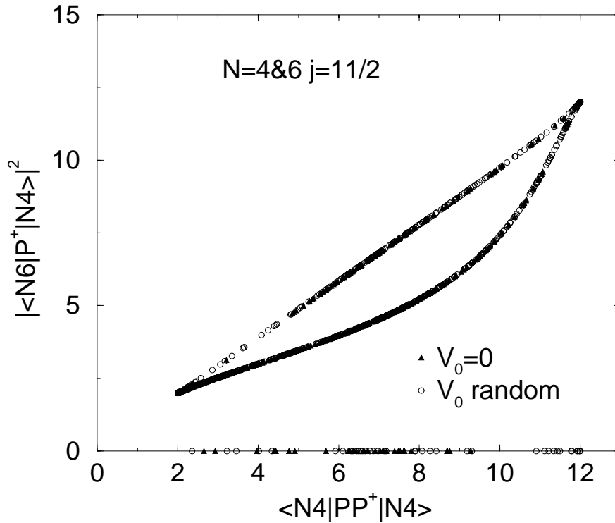
Figure 3.22: The numerator of f_p vs the denominator in eq. (3.31), evaluated for the N = 4 and 6, j = 11/2 systems with J_0 = 0 . P_0^\dagger creates a pair of particles coupled to spin zero. It acts on N = 4 , J = 0 ground states to make an N = 6 , J = 0 state which is overlapped with the ground state of the corresponding N = 6 system. The operator P_0^\dagger P_0 counts the number of pairs in the N = 4 state. Note the structure is unchanged by setting V_L = 0 , again the effect is geometric.
