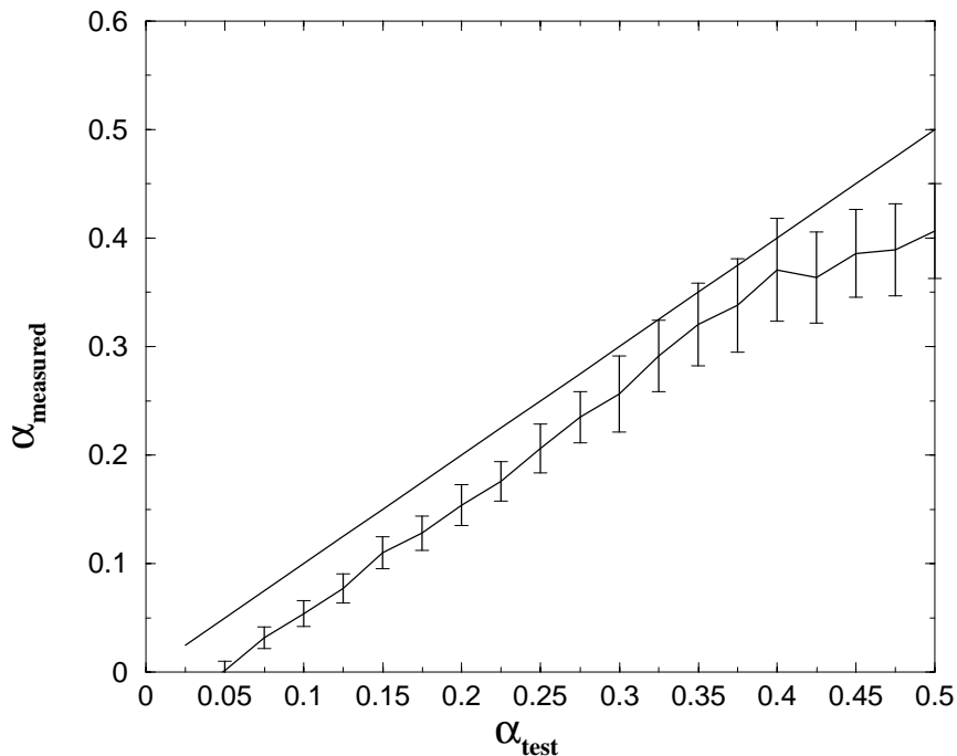
Figure 2.2: The procedure for extracting \alpha from P(s) was tested on GOE spectra ( N = 1000 ). The measured values \alpha_{measured} were systematically lower than the actual values \alpha_{test} by approximately 0.05. However the slope of the graph is unity up to a value of \alpha = 0.42
