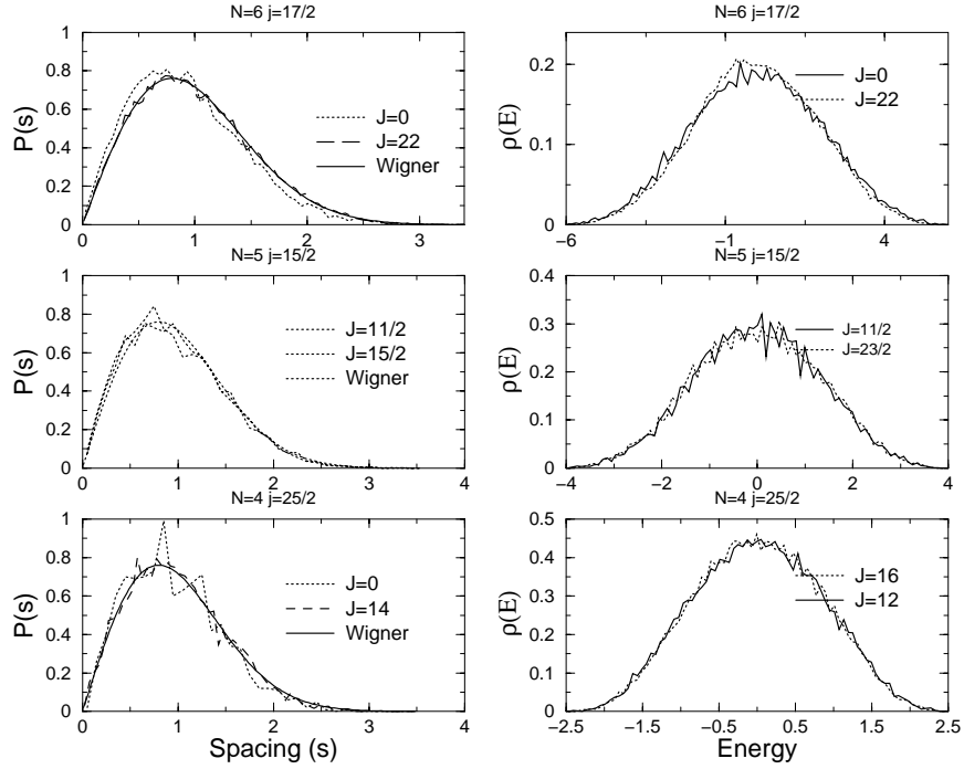
Figure 3.15: The distribution of energies, \rho_J(E) , (right panels), and energy spacings, P_J(s) , (left panels), with fixed J for three representative systems.
