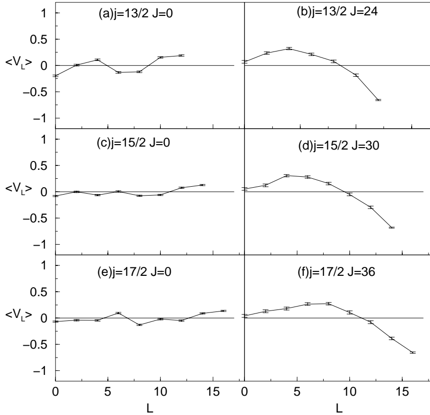
Figure 3.11: The mean value, \langle V_L \rangle , of the subsets of \{V_L\} vs. L that give J_0 = 0 or J_0 = J_{max} , for all the N = 6 systems. The panels are labelled with the value of the single-particle spin, j . On the left are the J_0 = 0 data, and on the right are the J_0 = J_{max} data.
