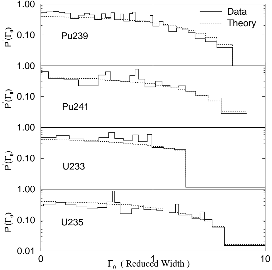
Figure 2.4: The distribution of reduced widths \Gamma^0 for all four data sets. The dotted line is P(x) = \chi^2(x|\nu = 1)
