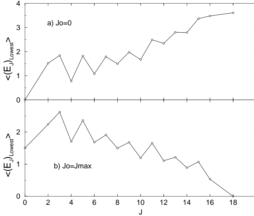
Figure 3.8: The average yrast line for a representative system, N = 6 , j = \frac{11}{2} .
