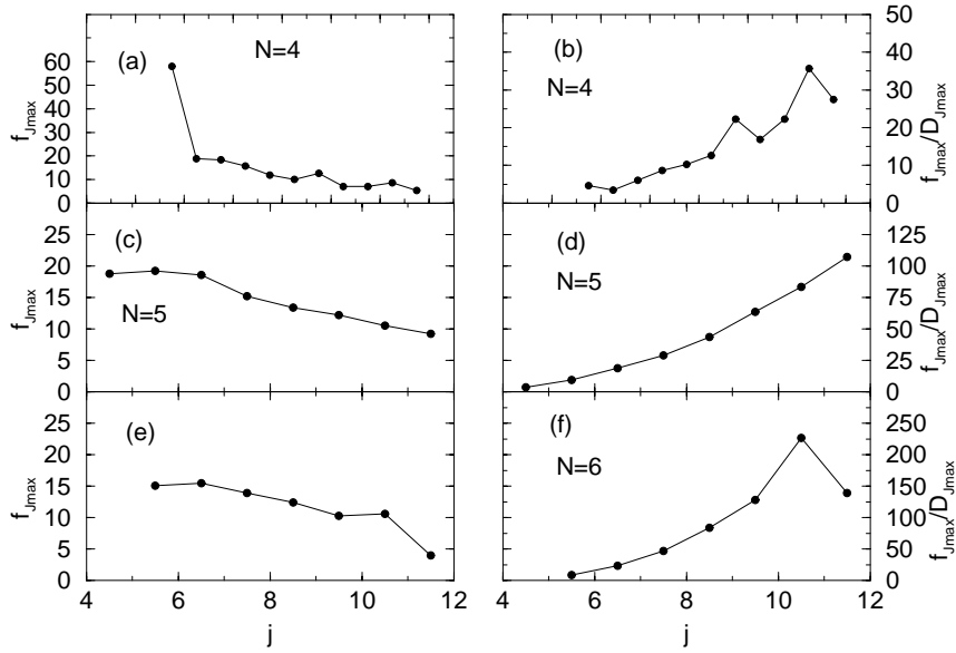
Figure 3.2: Same as Fig. 3.1 but this time we show f_{J_{max}}
