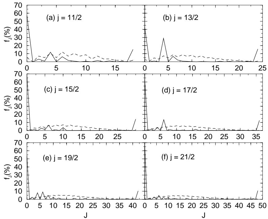
Figure 3.5: The distribution f_J of ground state spins J_0 for various systems of N = 6 particles.
