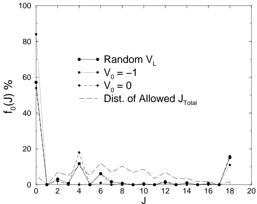
Figure 3.6: f_0 is shown for the N = 6 , j = \frac{1}{2} system. The cases where the pairing interaction are random or zero are practically indistinguishable.
