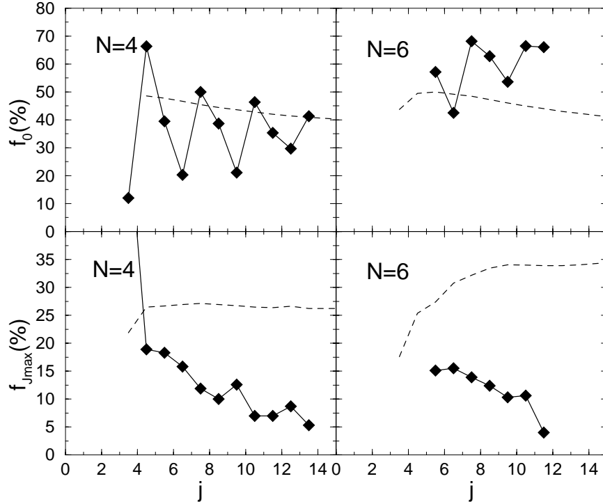
Figure 4.3: f_0 , the fraction of ground states with J = 0 , and (an upper boundary for) f_{J_{max}} for N = 4 , and 6 for different j . Ensemble results; solid line. Statistical theory; dotted line.
