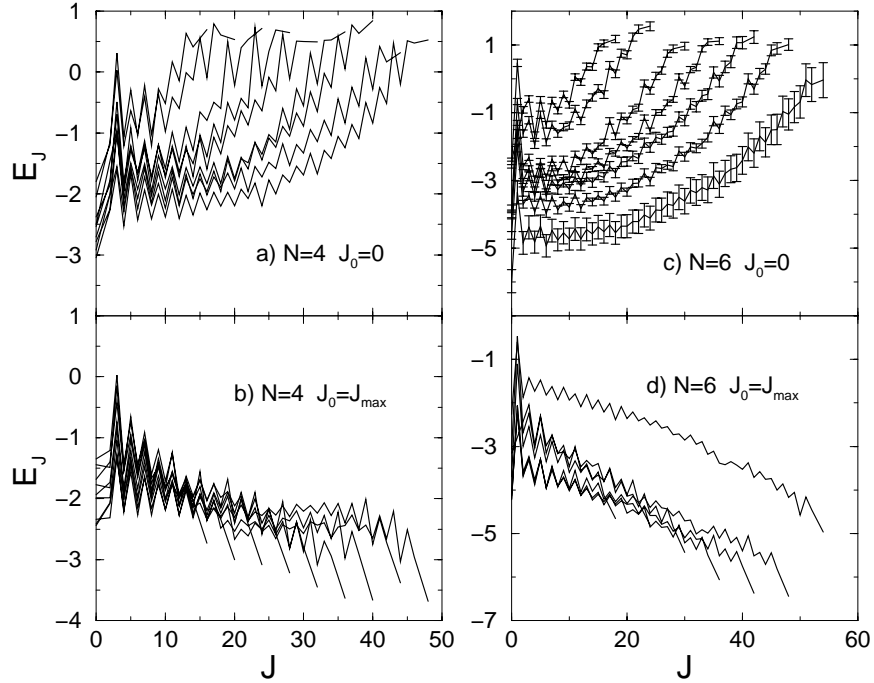
Figure 3.9: The average yrast lines for all the N = 4 and 6 particle systems. The range of j starts from 11/2 and goes to 27/2 for N = 4 , and 21/2 for N = 6 . The longer lines correspond to systems of higher j . Error bars for 3 panels have been omitted for clarity, but are comparable to those of the J_0 = 0 spectra.
