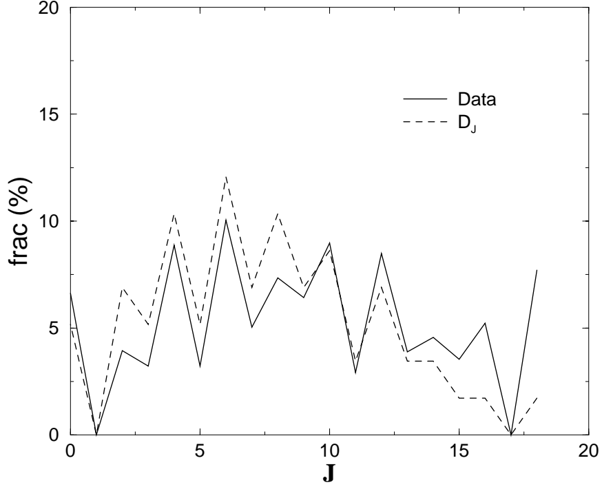
Figure 3.14: The fraction of systems with ground states spin J_0 = J vs J for fake spectra where \sigma(J) is taken from the N = 6 , j = 11/2 ensemble.
