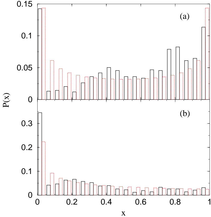
Figure 3.7: The distribution of overlaps, eq. 3.18, of ground states with J_0 = 0 with the fully paired (seniority zero) state are shown as solid histograms. Panel (a) corresponds to the ensemble with random V_{L \neq 0} and regular pairing, V_{L=0} = -1 . Panel (b) corresponds to the ensemble with all V_L random. Dashed histograms show the predictions for chaotic wave functions of dimension d = 2 , panel (a), and d = 3 , panel (b).
