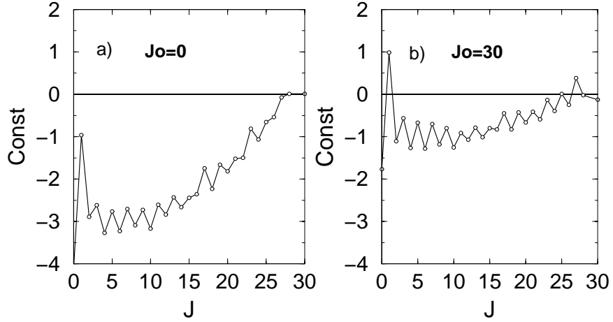
Figure 4.6: The constant shift in the theoretical equilibrium energies of spin J vs. J for the N = 6 j = 15/2 ensemble.
