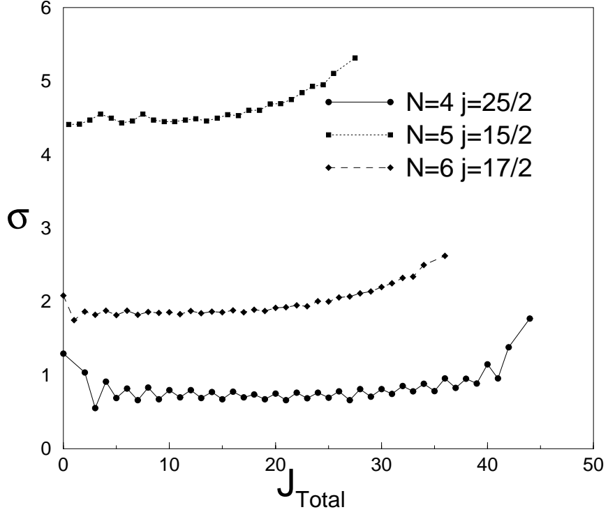
Figure 3.12: The standard deviation of the level density, \rho_J(E) , of states with total angular momentum J_{Total} for three representative systems.
