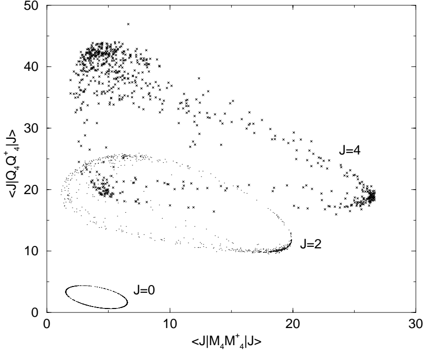
Figure 3.21: The quantities S_{Q;L}[J] and S_L[J] are strongly correlated for different values of J . This is just a geometric effect. The quantities are calculated for the lowest J states. Here N = 4 and j = 11/2 .
