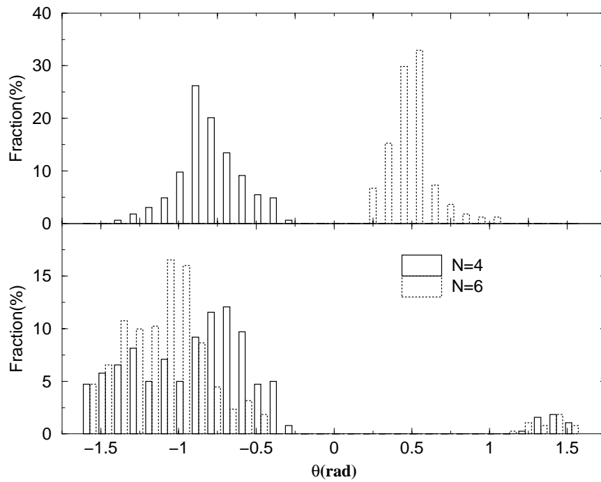
Figure 3.23: The distribution of the angles made by the J = 0 g.s. in the 2-dimensional space \{|S = 0\rangle, |S = 4\rangle\} for N = 4, 6 . Panel a) corresponds to those points on the straight line portion of Fig. 3.22 while panel b) is for those points on the curved part.
