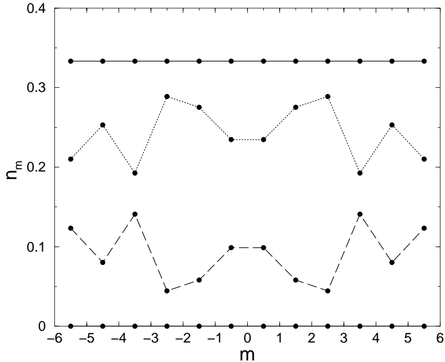
Figure 3.19: The contribution to the occupation numbers n_m of the |S = 0, N = 4\rangle state from Slater determinants of seniority 0, straight line. The jagged lines depict the decomposition of n_m for |S = 4, N = 4\rangle into contributions from seniority-4 (upper dotted line) and seniority-0 (lower dashed line) Slater determinants; here j = 11/2 .
