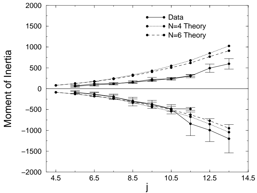
Figure 4.8: The moment of inertia for the N = 4 and 6 particle systems of a given j plotted as a function of j . The positive values are for the J_0 = 0 systems and the negative values correspond to the J_0 = J_{max} systems.
