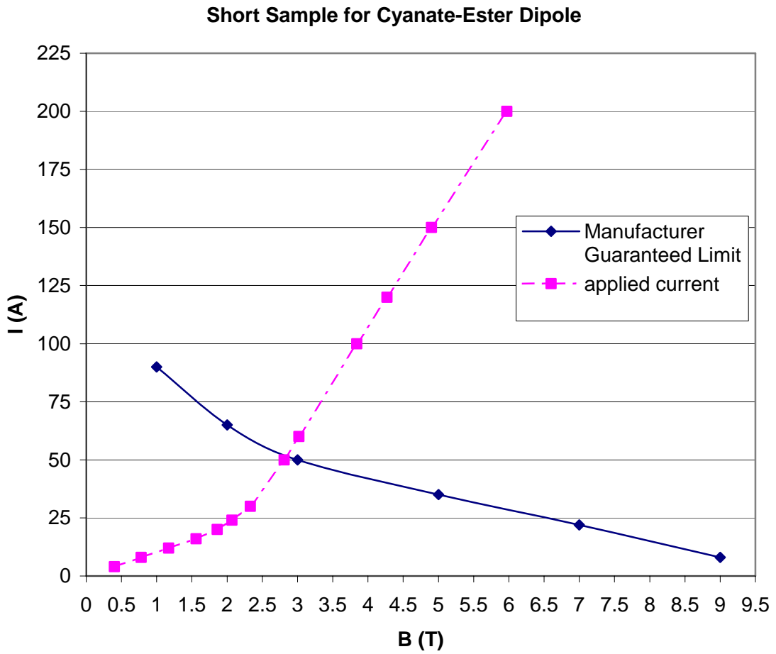
Fig. 2-4: The short sample current limit guaranteed by the manufacturer (Supercon, Shrewsbury, MA) is plotted along with the field (at the conductor) and required current calculated by POISSON [Ref. 13]. Their intersection, about 50 amps, is the estimated short sample current of the magnet [Ref. 4].
