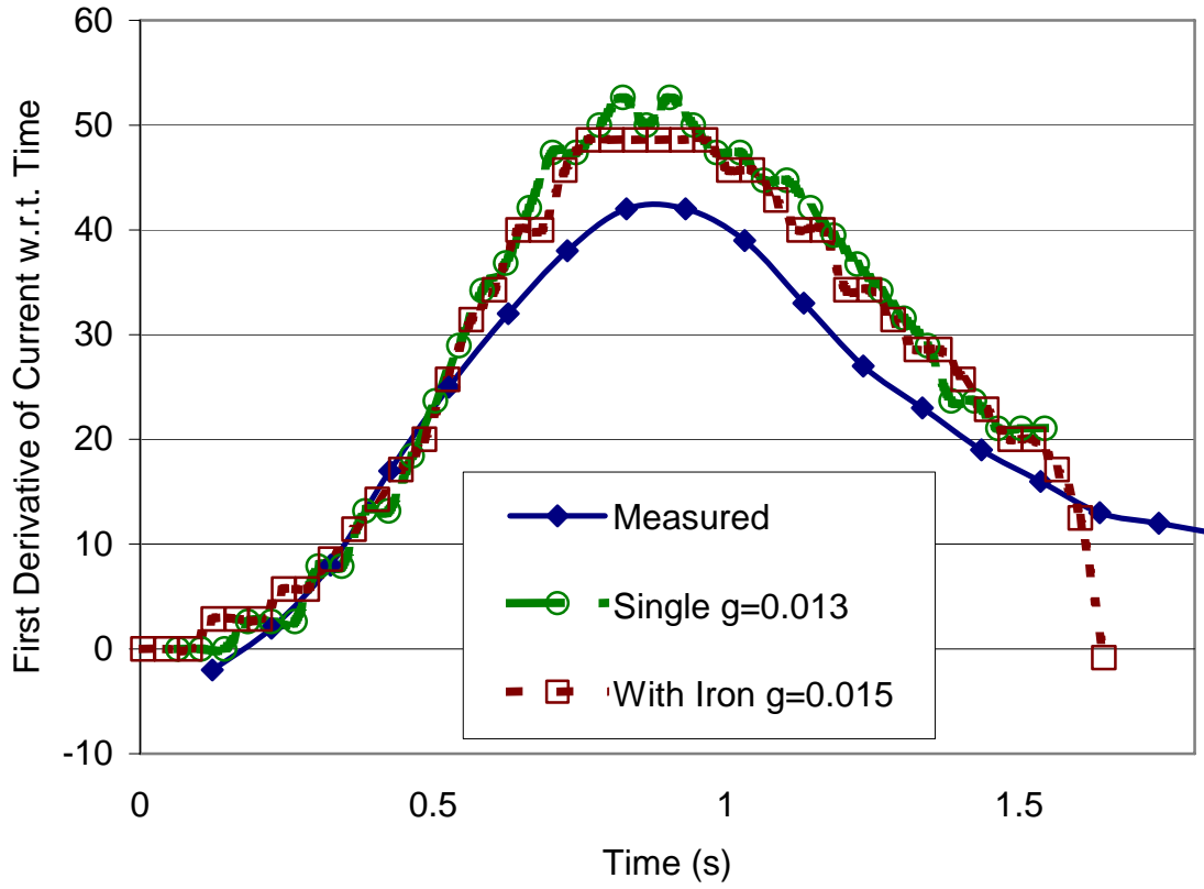
First Derivative of Current for Cyanate-ester Dipole
