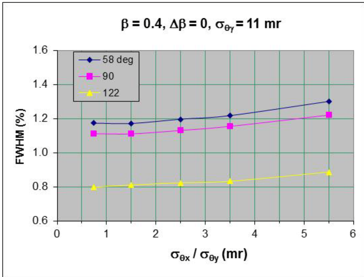
Figure 2: Energy resolution of GRETINA after Doppler-shift reconstruction for \gamma -rays emitted at 0.4c. No effects other than the spatial resolution of GRETINA are taken into account. The x-axis shows the dependence with the uncertainty \sigma_{\theta_x} , \sigma_{\theta_y} of the projectile's scattering angle.
